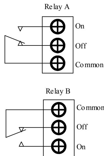
Figure 2 Terminal Connectors
